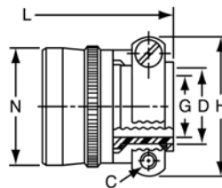
"A" (SR), "E" (SR), "P" (SR) Strain Relief
