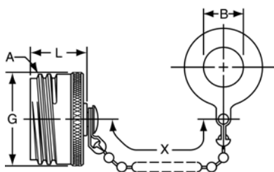
PLUG PROTECTION CAP FOR PC CONNECTORS 10-101955-XXX
