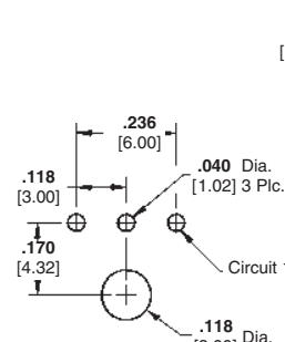
Recommended PC Board Layout 3 Position*
