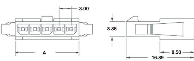
Receptacle housing, panel mount, single-row
