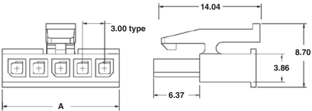
Plug housing, single row
