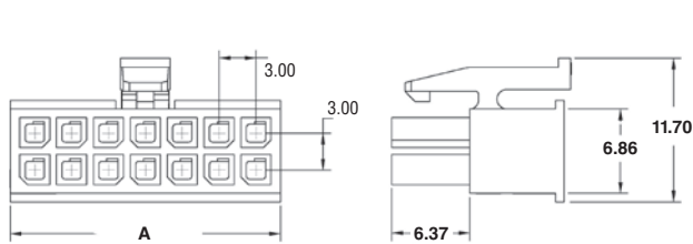
Plug housing, multi-row
