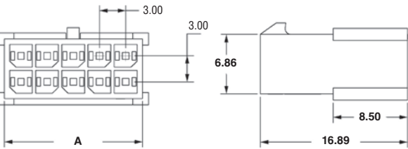
Receptacle housing, multi-row, free hanging
