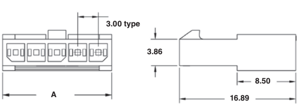
Receptacle housing, single-row, free hanging
