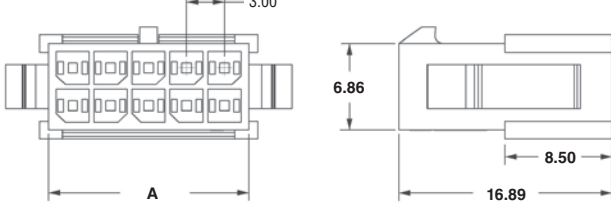
Receptacle housing, panel mount, multi-row
